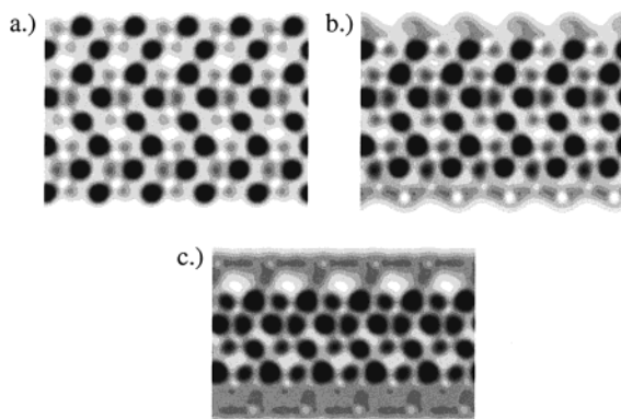
Figure 5. Vertical cut through valence electron density of the (relaxed) stoichiometric and Al-rich terminations of alumina where (a) is (1 × 1) stoichiometric, (b) has one oxygen layer removed, and (c) has two oxygen layers removed on each side of the slab. There are 10 contours spanning a range of 0–1. The dark areas are where the oxygen anions reside.
